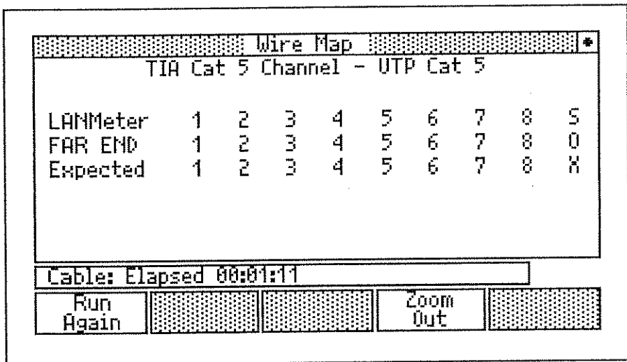
Figure 4-11. Wire Map Autotest Sample Results
